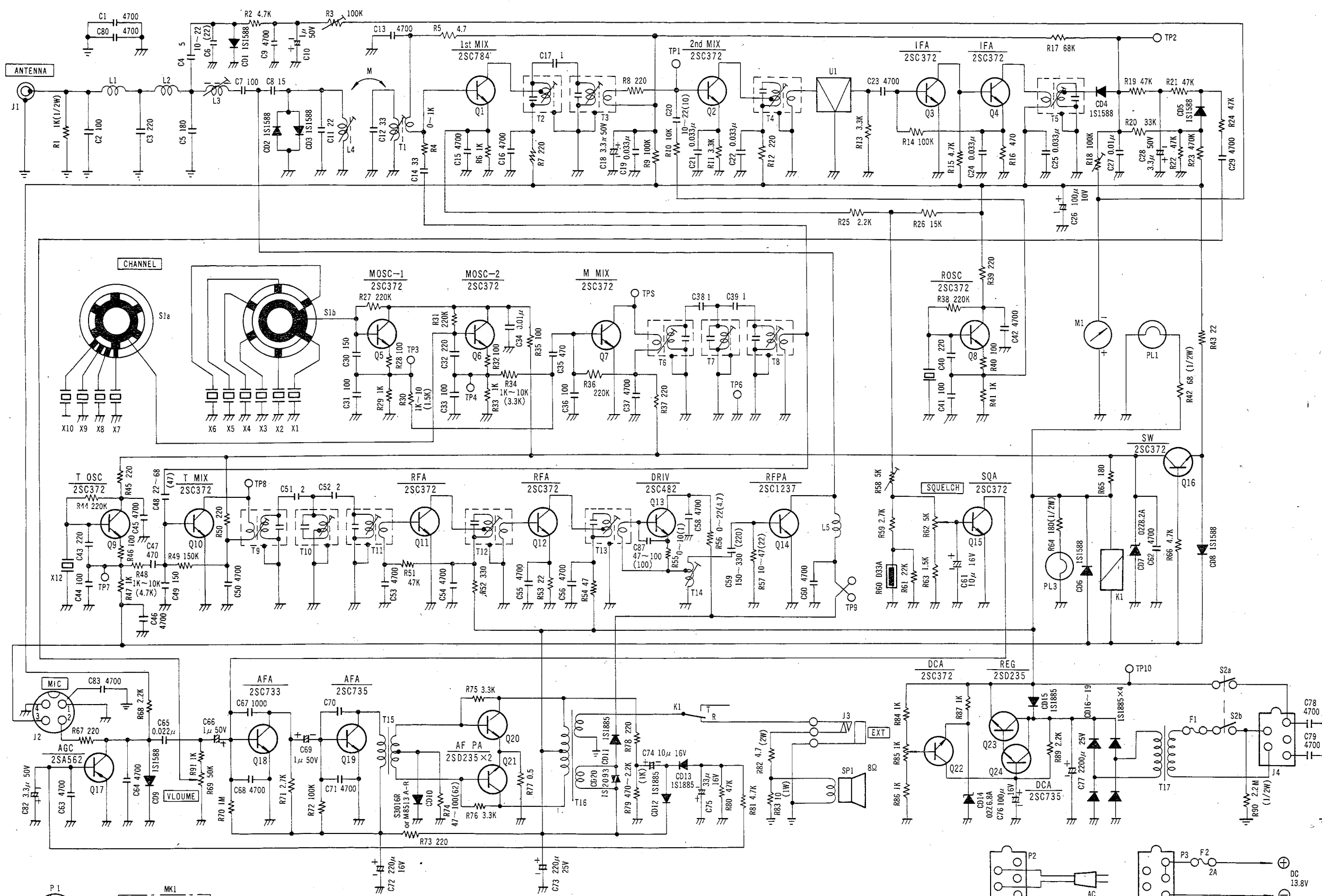
SCHEMATIC COBRA 85 480-164-9-001
